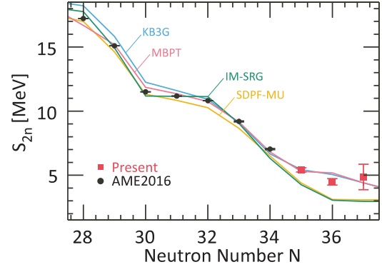
Fig. 1. The two-neutron separation energies in neutron-rich Ca isotopes. Squares indicate values determined for the first time, and circles are literature values from AME2016. 6) The solid lines show theoretical predictions. 7-10)
